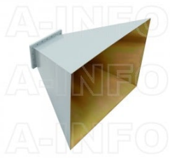
LB-975-15-A Standard Gain Horn Antenna 0.75-1.12GHz 15dB Gain Rectangular Waveguide Interface
