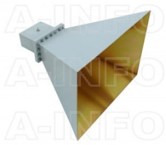
LB-975-15-C-SF Standard Gain Horn Antenna 0.75-1.12GHz 15dB Gain SMA Female
